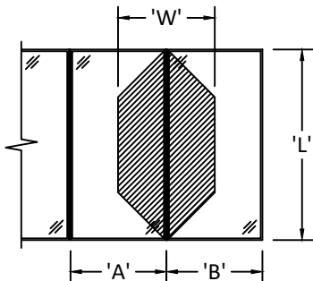
ONE-WAY MULLION DIAGRAM
