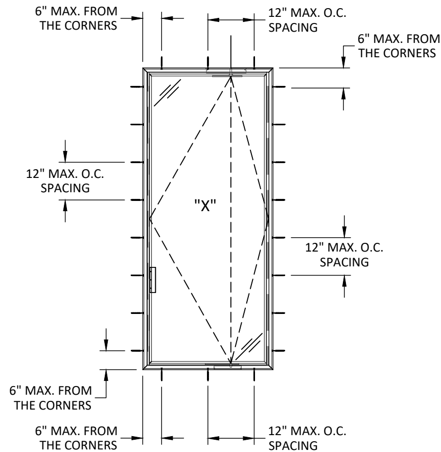
"X" ANCHOR LAYOUT THROUGH FRAME INSTALLATION
