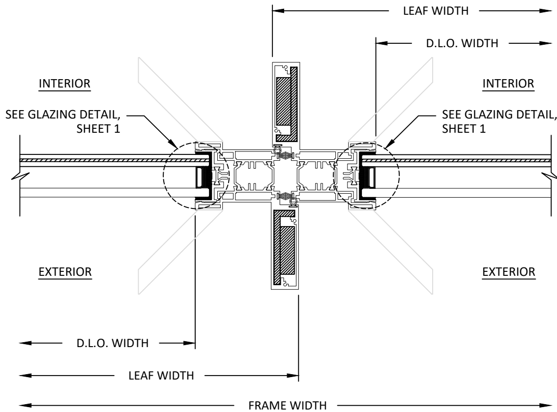
B 8 HORIZONTAL SECTION MEETING STILE
