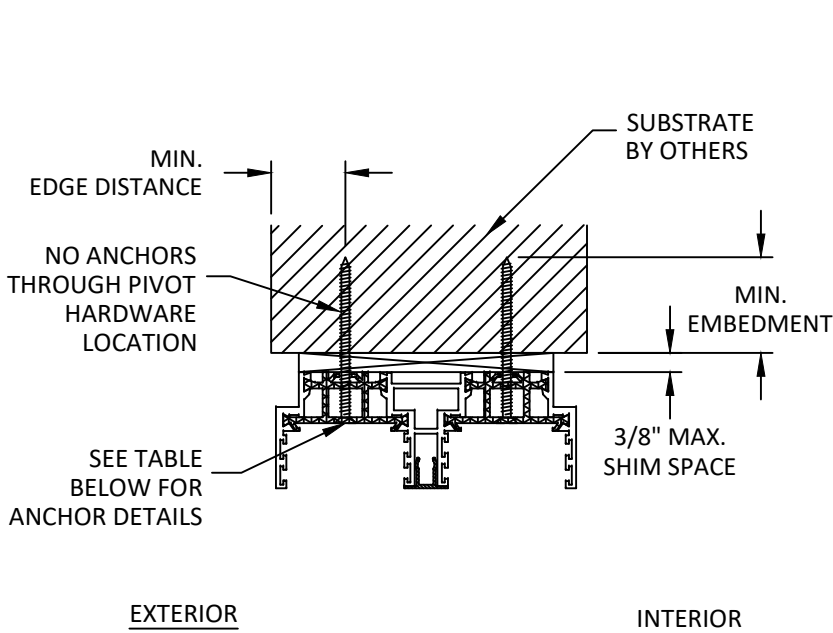
A 9 VERTICAL SECTION HEAD - THROUGH FRAME NOTE: SIDELITE HEAD & SILL SIMILAR
